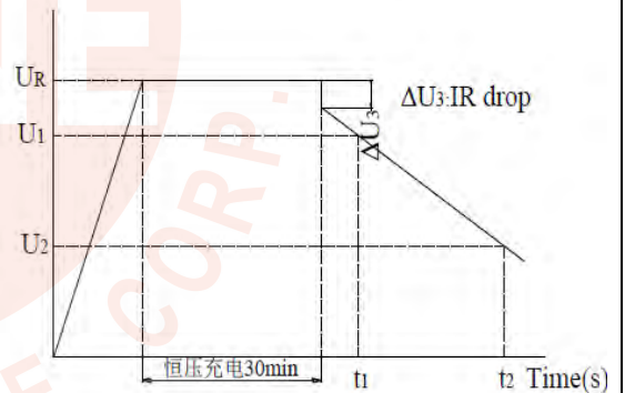
Figure 2. Charge and Discharge Curve Diagram.
