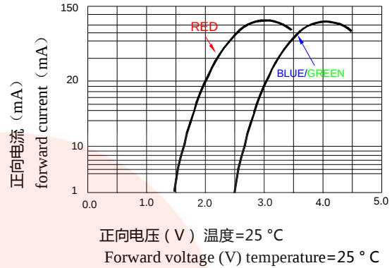
正向电压与正向电流的关系 The relationship between forward voltage and forward current
