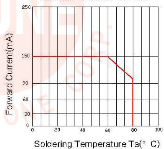
Soldering Temperature VS. Forward Current
