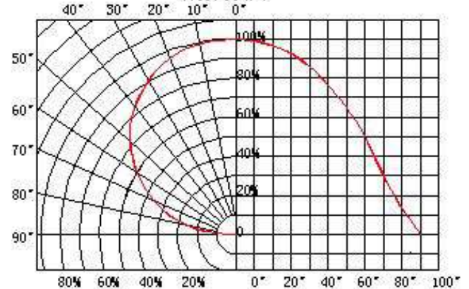
Radiation diagram
