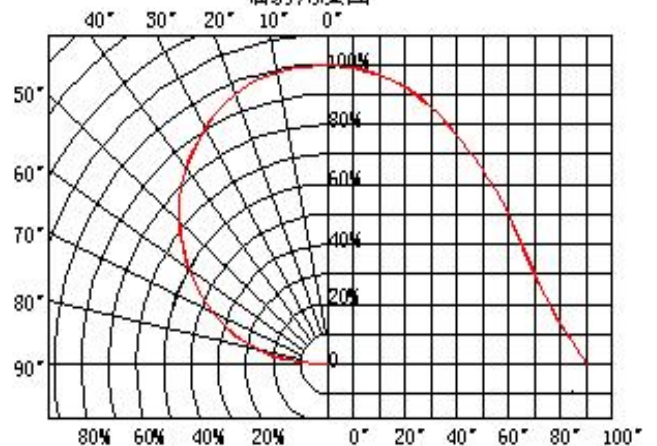
Radiation diagram
