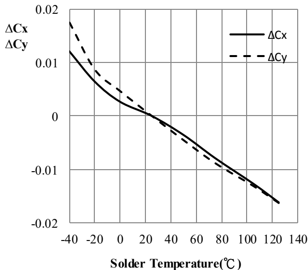
Chromaticity Coordinate vs. Solder Temperature
