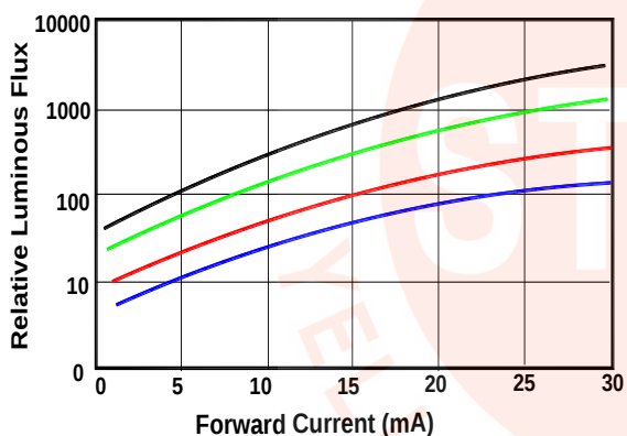
5). Electrical Characteristics
