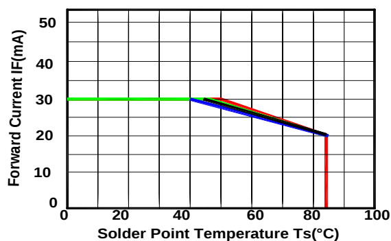
8). Thermal Design(R/G/B/W 1 chip on light)
