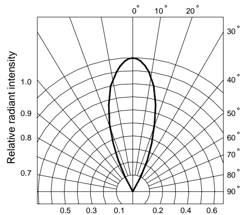
Fig.6 Radiation diagram
