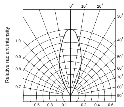
Fig.6 Radiation diagram
