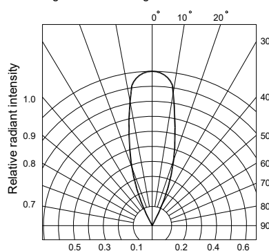
Fig.6 Radiation diagram
