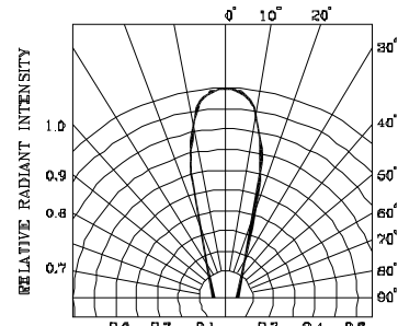
RADIATION DIAGRAM
