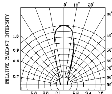
RADIATION DIAGRAM
