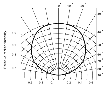
Fig.6 Radiation diagram
