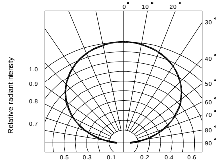
Fig.6 Radiation diagram
