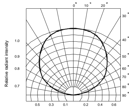
Fig.6 Radiation diagram
