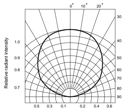
Fig.6 Radiation diagram
