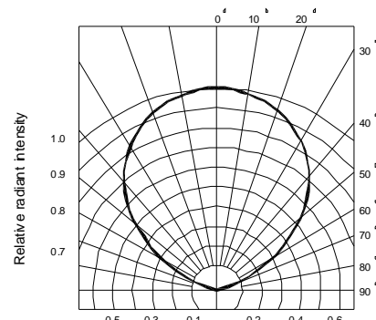
Fig.6 Radiation diagram
