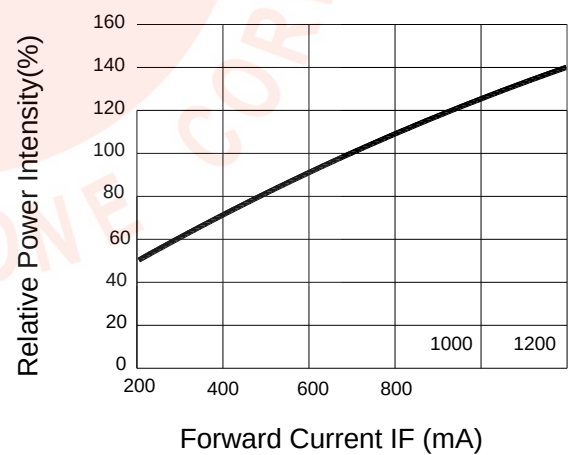
Relative Radiant Flux VS. Forward Current
