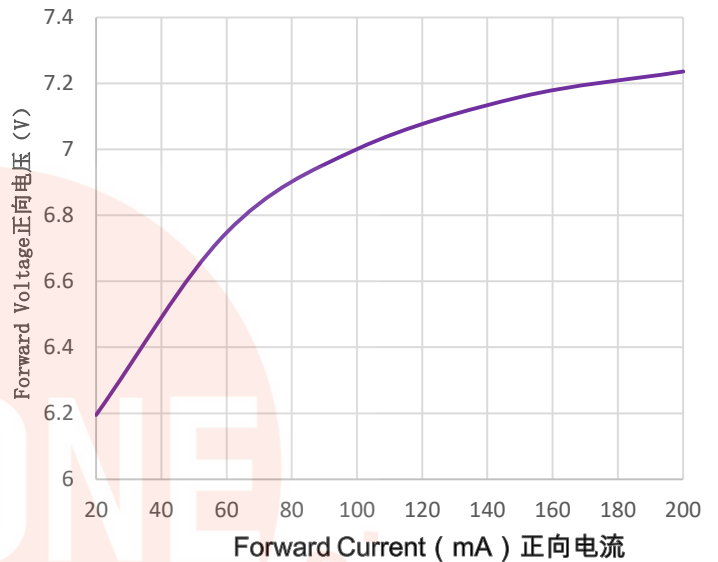
(2) I-V特性 I-V Characteristic
