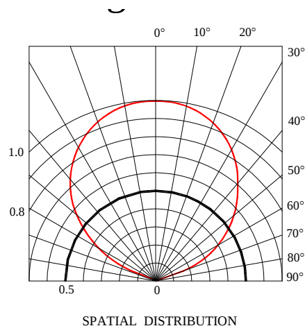
SPATIAL DISTRIBUTION
