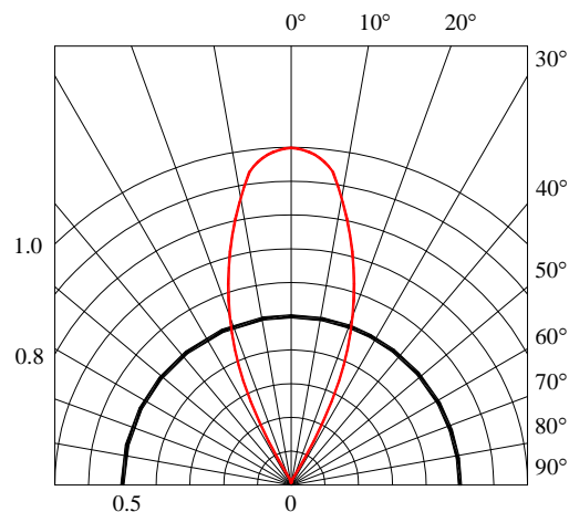
SPATIAL DISTRIBUTION
