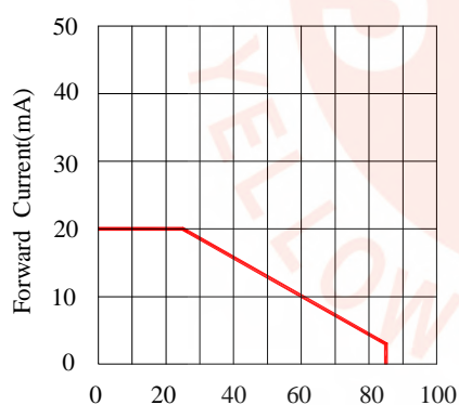
Ambient Temperature(°C) FORWARD CURRENT DERATING CURVE
