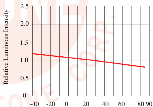
Ambient Temperature(°C) LUMINOUS INTENSITY Vs. AMBIENT TEMPERATURE
