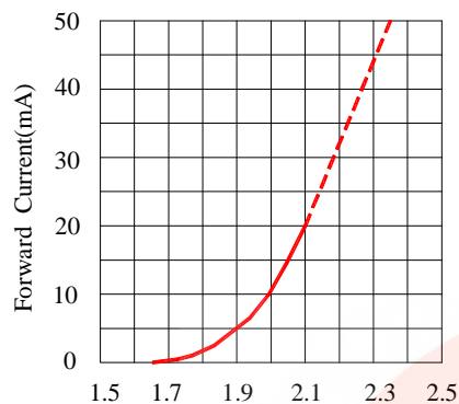
Forward Voltage(V) FORWARD CURRENT Vs. FORWARD VOLTAGE
