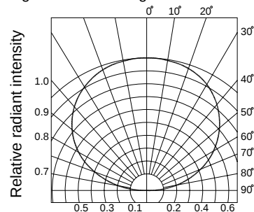
Fig.6 Radiation diagram
