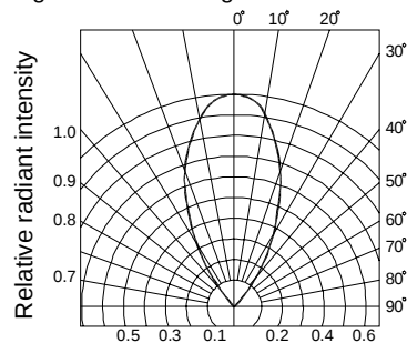
Fig.6 Radiation diagram
