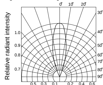
Fig.6 Radiation diagram
