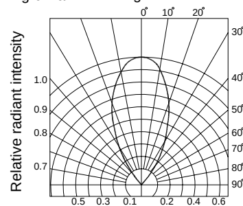
Fig.6 Radiation diagram
