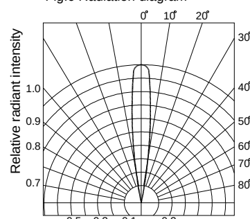
Fig.6 Radiation diagram
