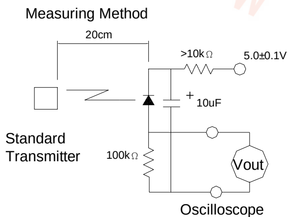
Fig.2 Measuring Method
