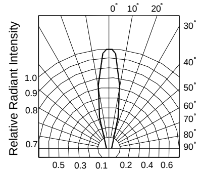
FIG.6 Radiant Diagram
