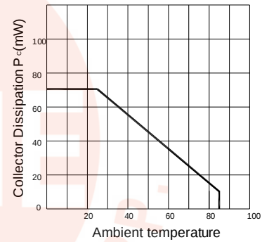
Fig.2 Ambient temperature vs. Collector Dissipation
