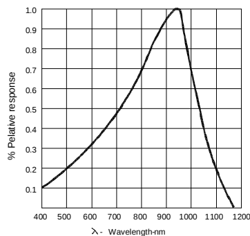
Fig.5 Relative spectral response
