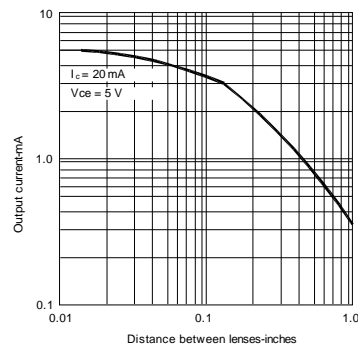
Fig.6 Coupling characteristics
