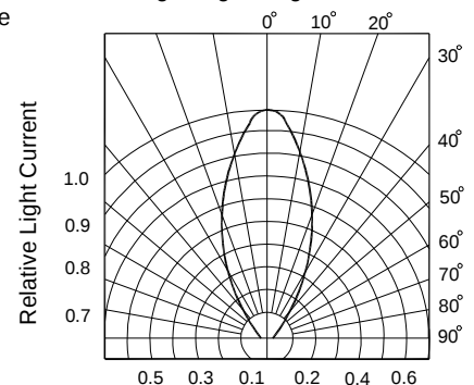
Fig6.Angle Diagram
