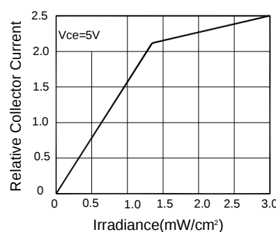
FIG.5 Relative Collector Current Vs. Irradiance
