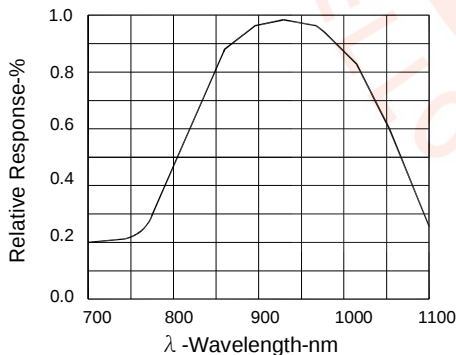
FIG.1 Relative Response vs.Wavelength
