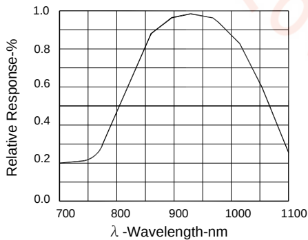
FIG.1 Relative Response vs.Wavelength
