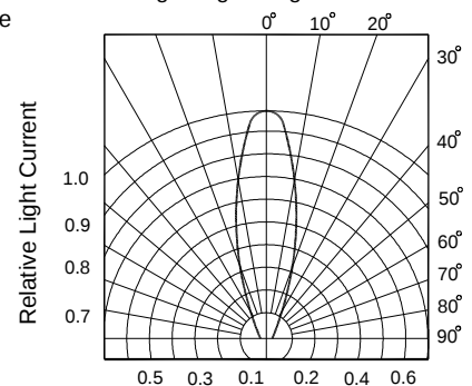
Fig6.Angle Diagram
