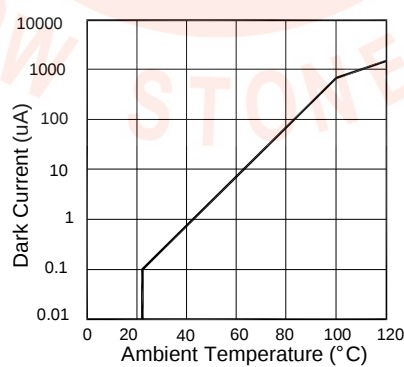
FIG.2 Dark Current Vs. Ambient Temperature
