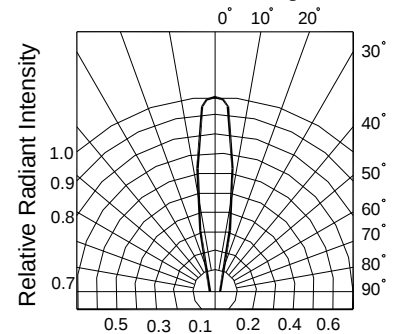
FIG.6 Radiant Diagram
