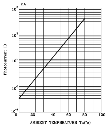
Fig.5 DARK CURRENT VS. AMBIENT TEMPERATURE mVR=10, Ee=0mw/cm 2
