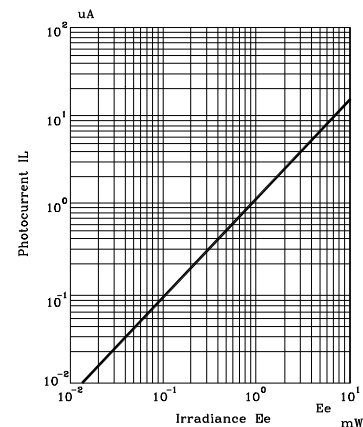
Fig.6 PHOTOCURRENT VS IRRADIANCE = 940 nm
