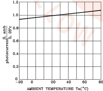
Fig.3 PHOTOCURRENT VS. AMBIENT TEMPERATURE
