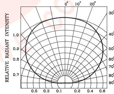
Fig.4 RADIATION DIAGRAM
