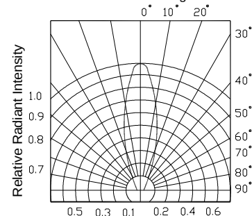
FIG.8 Radiant Diagram
