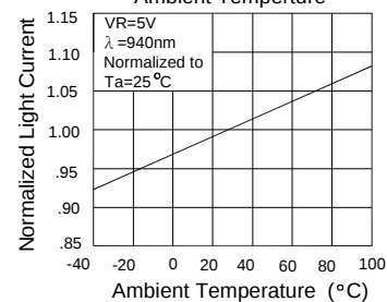
Fig5.Normalized Light Current vs Ambient Temperature
