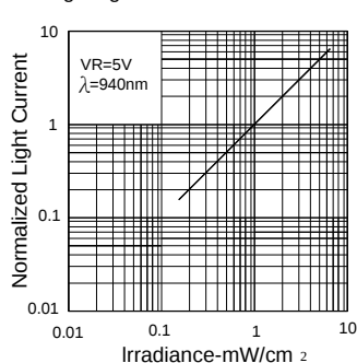
Fig6.Light Current vsIrradiance
