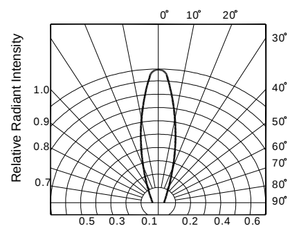
FIG.6 Radiant Diagram
