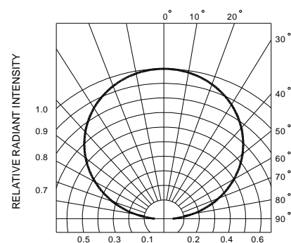
RADIATION DIAGRAM
