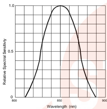
Fig.1 Relative spectral sensitivity vs wavelength
