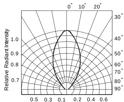
FIG.6 Radiant Diagram
