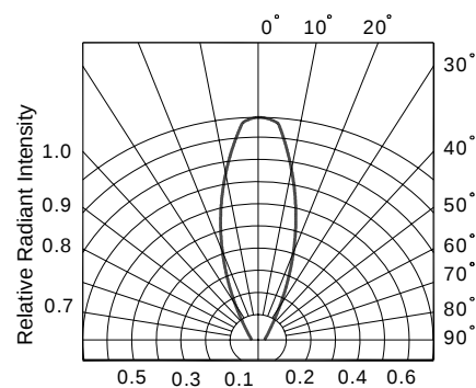
FIG.6 Radiant Diagram
