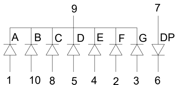
Common Cathode( YDS-31214CR-N )
