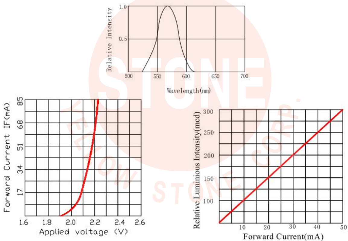
Forward Current Vs. Relative luminous Intensity
