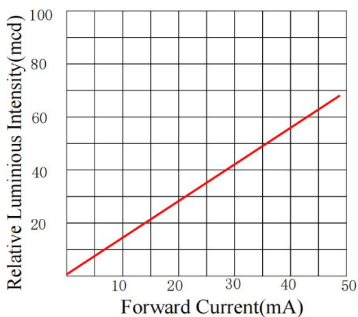
Forward Current Vs Relative luminous Intensity
