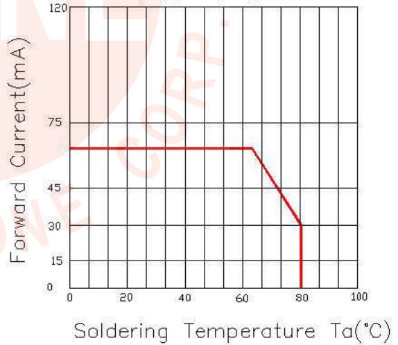
Soldering Temperature VS. Forward Current
