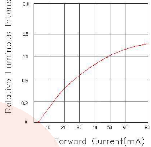
Forward Current VS. Relative Intensity
